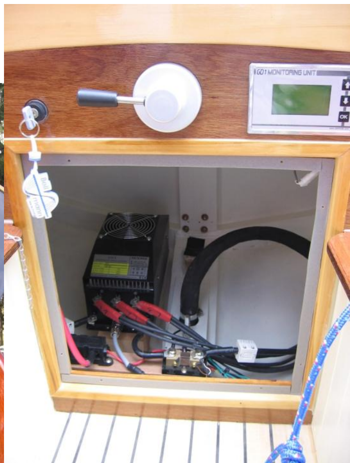
4.2kW Pod motor installed on classic timber launch
